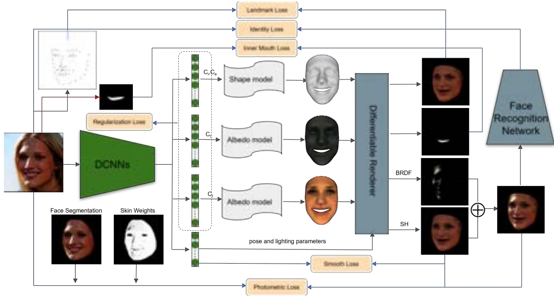
Figure 2: Schematic view of our method. We use the ResNet-50 (DCNNs) [21] as the backbone of our network.
