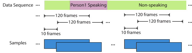
Figure 3: Illustration of data sample generation in this work. Each sample contains 120 frames with 110 frames overlapped with the previous/next samples.
