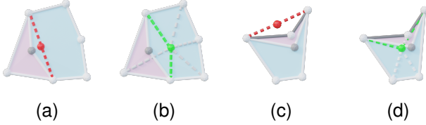
Fig. 10: (a) The traditional approach creates a flat corner due to the lack of edge connectivity to the red node. (b) By considering all one-ring neighbor vertices, the vertex moves toward the centroid, which creates a convex quad face. (c) On the boundary, the traditional approach creates inverted cells since the vertex position moves outside the boundary. (d) With the adjusted approach, the vertex remains inside the boundary.
