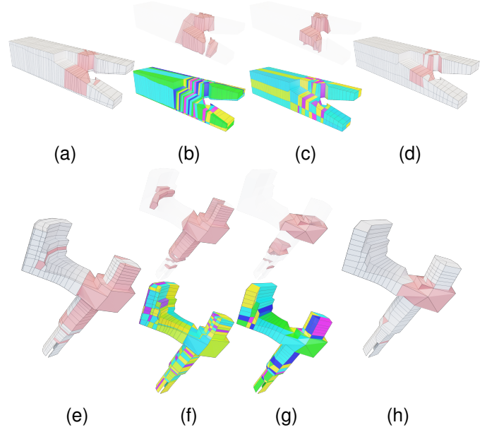
Fig. 12: Two meshes with the LoopyCuts approach [3]. The top row shows the halved_oblique_scarf_2_mm model (a), its non-hex cells (b, top), and hybrid base complex (b, bottom). After simplification (d), the remaining non-hex cells (c, top) lead to a simpler hybrid base complex (c, bottom). The bottom row shows the nugear_mm model (e), its non-hex cells (f, top), and hybrid base complex (f, bottom). After simplification (h), non-hex cells in the L-shaped region are fully removed (g, top), yielding a much simpler hybrid base complex (g, bottom).
