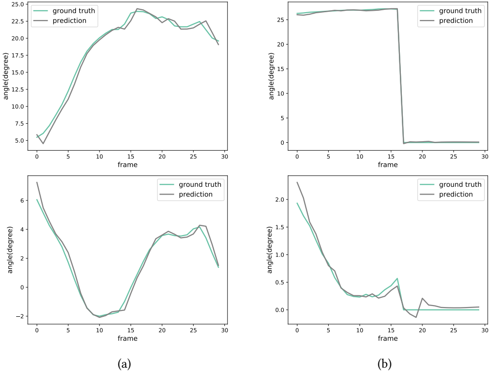
Fig. 6. (a) A test result for the speaker LSTM model: the top panel is the yaw angle \alpha , the bottom is the pitch angle \beta , and (b): A test result for the listener LSTM model, the top panel is the yaw angle \alpha , the bottom panel is the pitch angle \beta .
