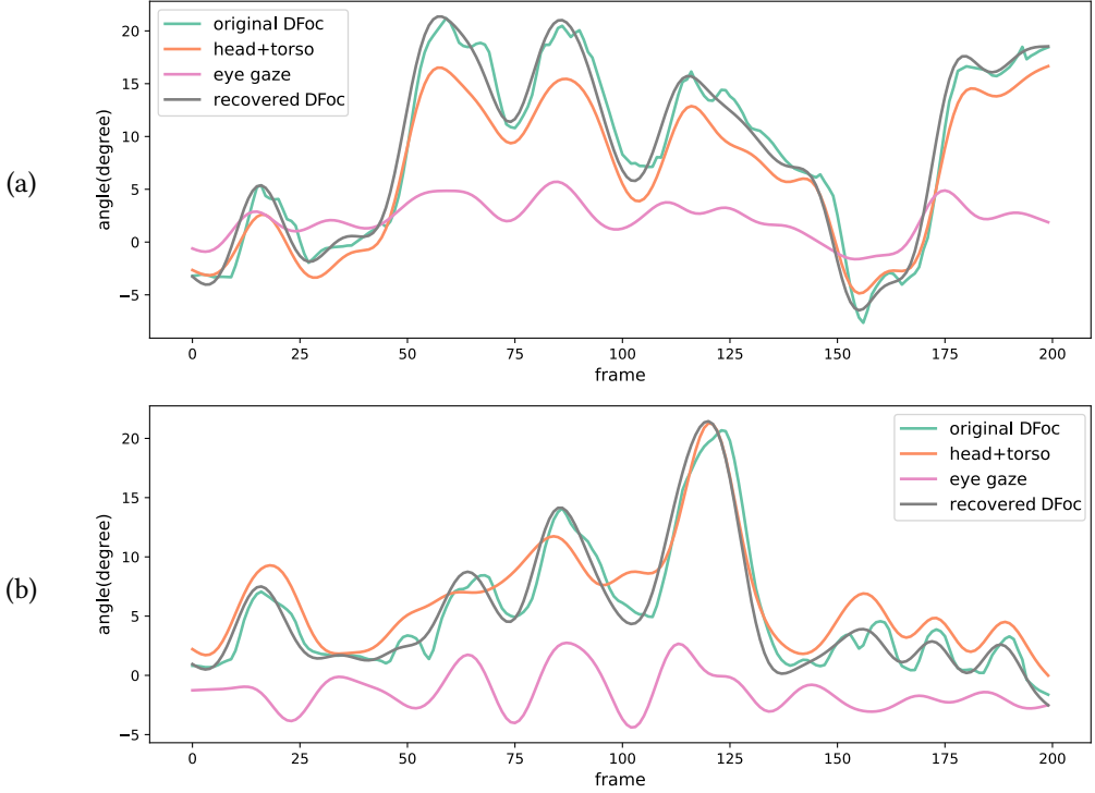
Fig. 8. Example results of the DFoc decomposition in our method. (a) The decomposed Yaw angles \alpha by our method. (b) The decomposed Pitch angles \beta by our method.
