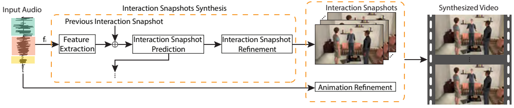
Fig. 3. Schematic view of our approach. It generates interaction snapshots frame by frame. This figure uses the generation of the i -th frame as an example. The system consists of two main components: interaction snapshots synthesis, and animation refinement. The color blocks on the input audio mark the speaking time of different interlocutors: the pink block for the left interlocutor, the green block for the middle interlocutor, and the yellow block for the right interlocutor.
