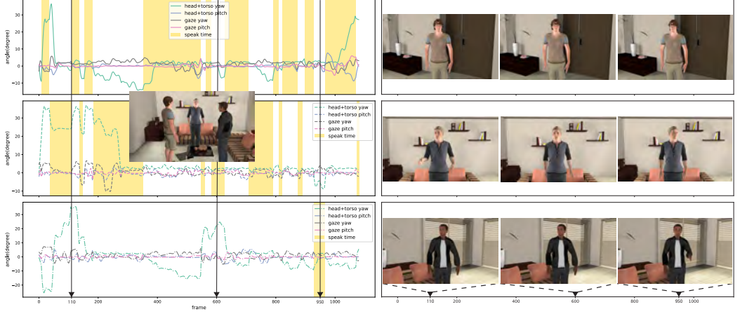
Fig. 10. The visualization of a synthesized three-party conversation example by our approach: the head+torso and gaze angles (including the yaw angle \alpha and the pitch angle \beta ) with their speak time. Each panel (from top to bottom) shows the information of one interlocutor. The snapshots in the right show the rendered corresponding interlocutor at three selected time frames.
