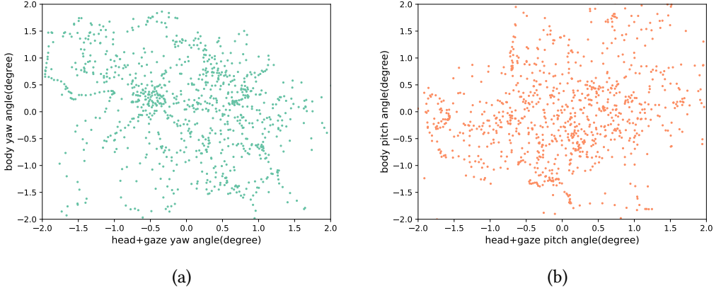
Fig. 9. Plotting of randomly selected, 10-min data samples (the combined directions of the head+gaze vs. the directions of the torso) in our dataset. (a) samples of the yaw angle \alpha , and (b) samples of the pitch angle \beta .
