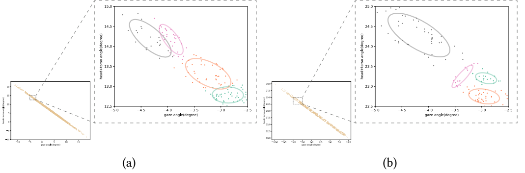
Fig. 7. (a): Samples in a bin ( 10^\circ - 11^\circ ) of the Yaw angle \alpha , and (b): Samples in a bin ( 19^\circ - 20^\circ ) of the Pitch angle \beta .
