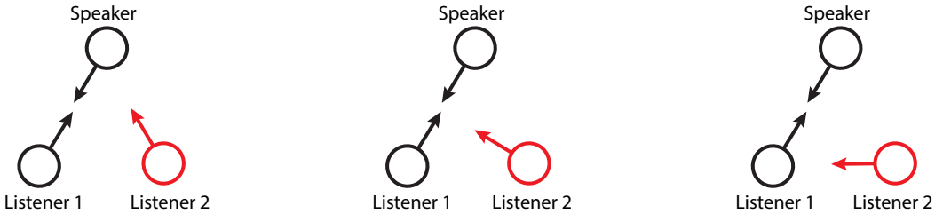
Fig. 4. Top views of some interaction snapshots that could occur in three-party conversations. The interaction snapshot in the left can be synthesized with existing two-party listener models. However, other two interaction snapshots can only be synthesized by our approach.
