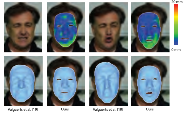
Fig. 17. Comparisons between our method and the reconstructed mesh (considered as the ground-truth) by the binocular method [19]. The top row shows the input image and the corresponding per-vertex error map. The bottom row shows the mesh comparisons.
