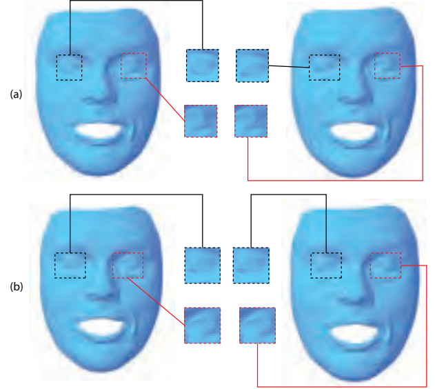
Fig. 9. A wrinkle transfer comparison between using Eq. 14 and using Eq. 15. (a) shows the wrinkles on two consecutive frames are transferred using Eq. 14, (b) shows the wrinkles on the same two continuous frames are transferred using Eq. 15.
