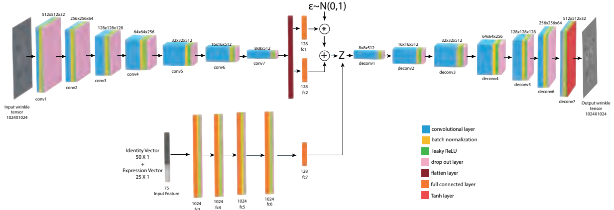
Fig. 3. Our network architecture overview. Our VAE consists of an encoder and a decoder, the encoder takes wrinkle tensors as inputs, and the decoder is able to generate wrinkle tensors. Our wrinkle embedding network aims to sample the latent space z , therefore, the decoder of the VAE can produce corresponding wrinkle tensors.
